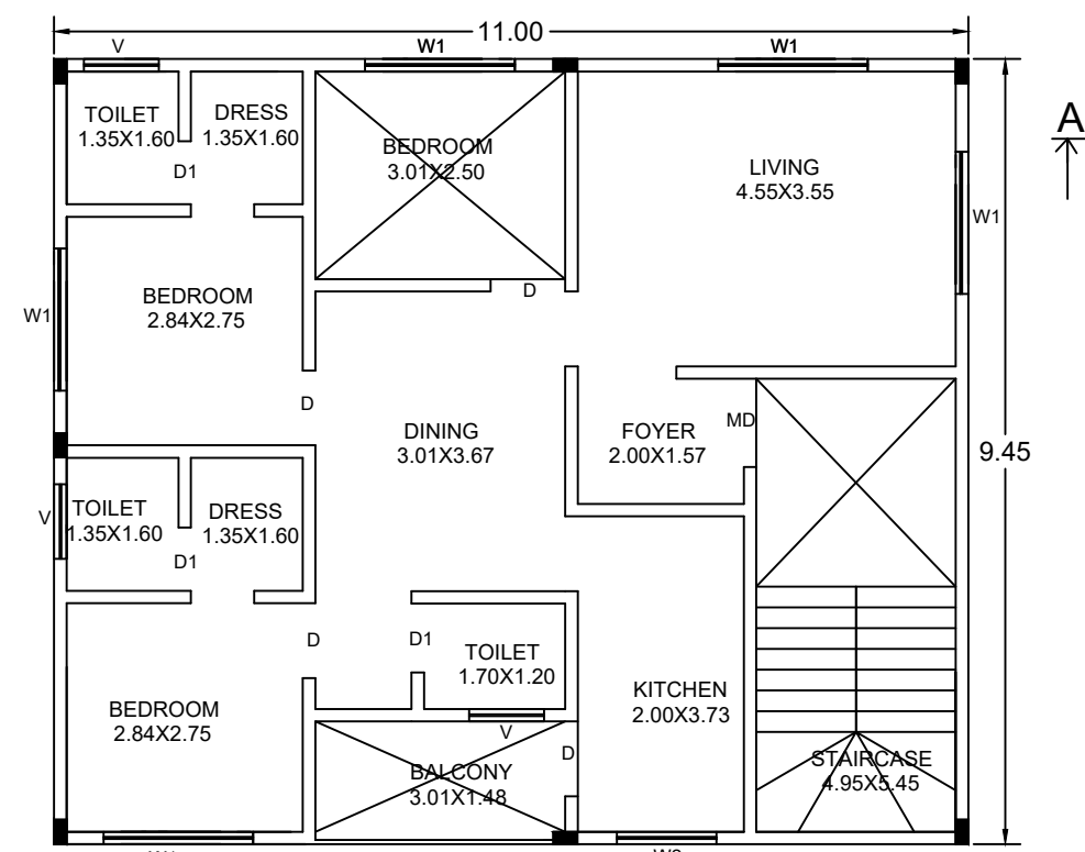
TYP: SECOND & THIRD FLOOR PLAN
